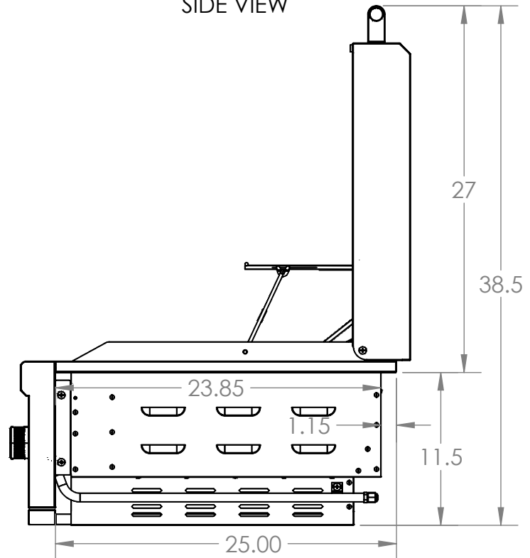
CRITICAL DIMENSIONS
