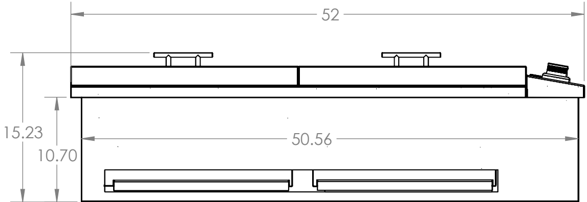
SIDE VIEW
