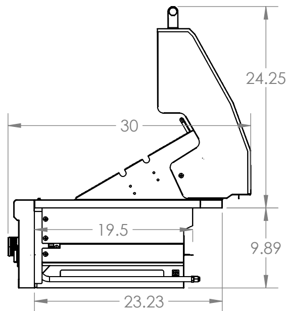
CRITICAL DIMENSIONS
